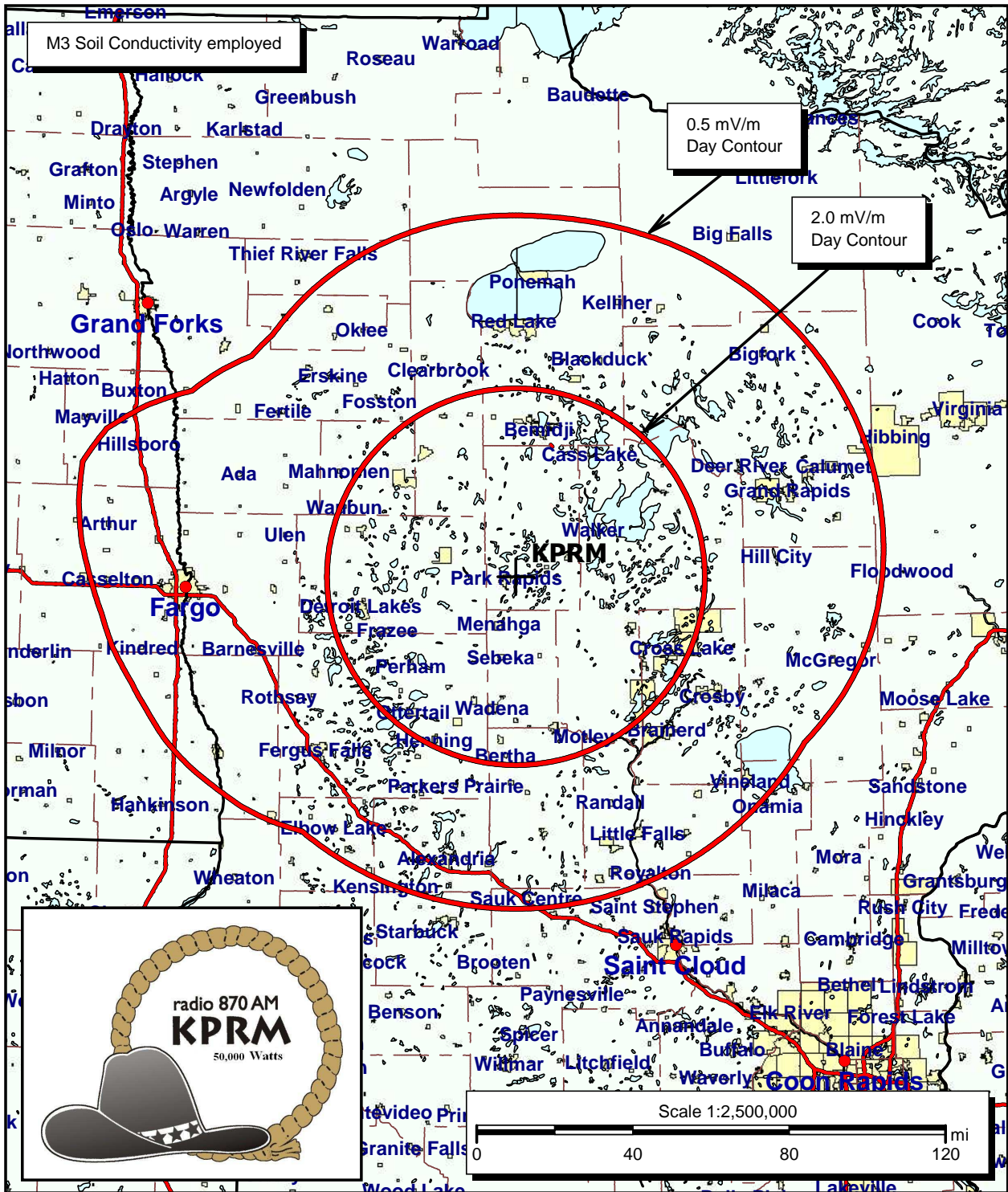
DAYTIME COVERAGE CONTOURS KPRM(AM) - 870 KHZ - PARK RAPIDS, MINNESOTA 50,000 WATTS DAYTIME/1,000 WATTS NIGHTTIME - DA-N
